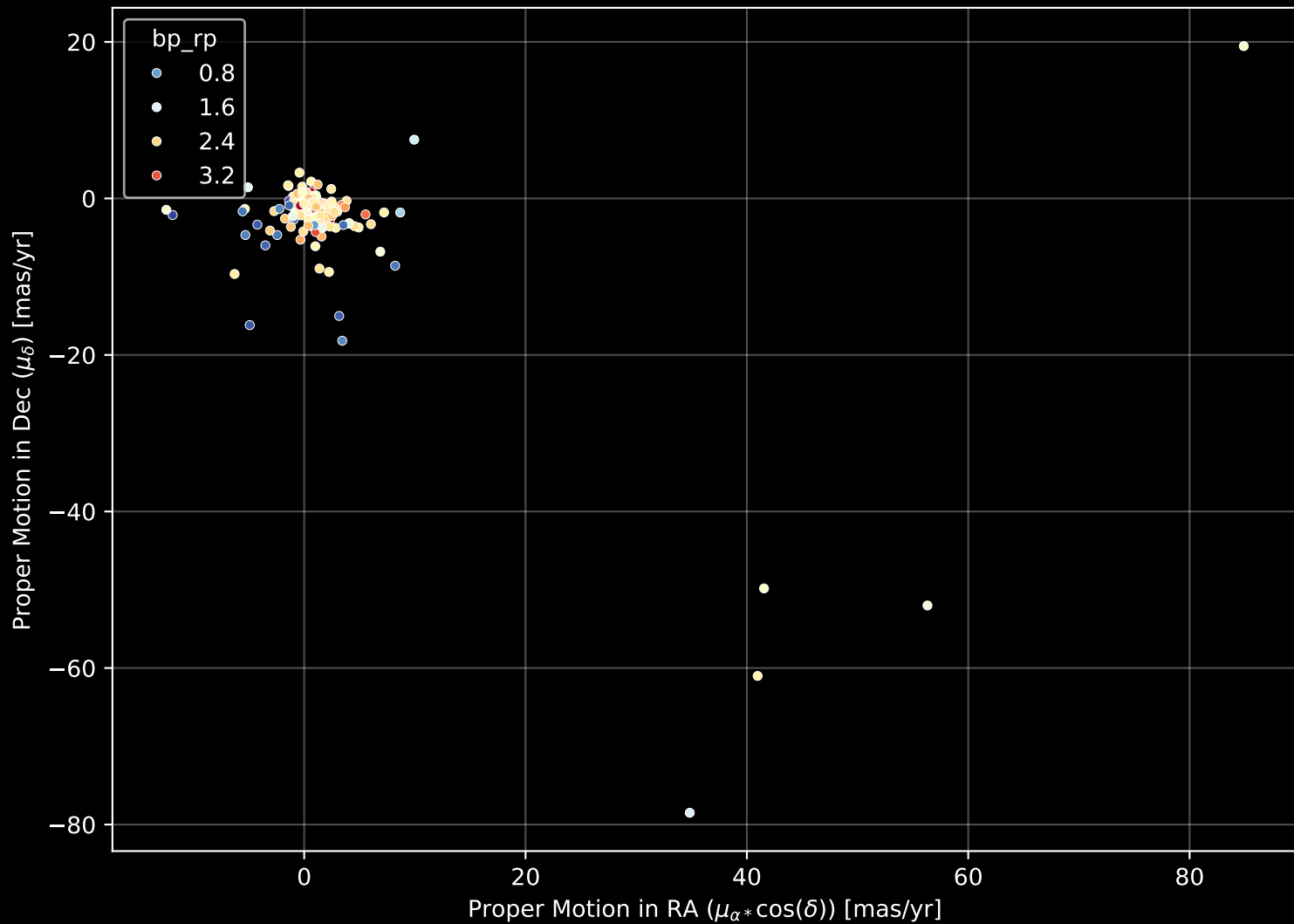
APOGEE DR17 Field: [154+04] Proper Motion Diagram (n= 190)
