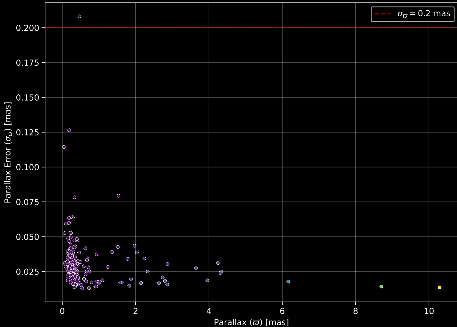
APOGEE DR17 Field: [154+04] Parallax Quality (n= 190)
