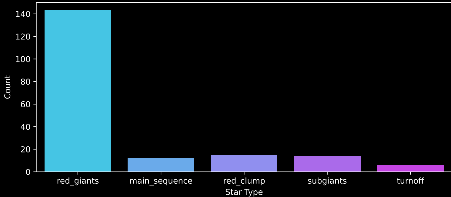
APOGEE DR17 Field: [154+04] Count plot of Star Type
