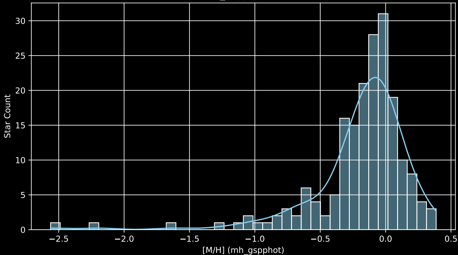
APOGEE DR17 Field: [154+04 [M/H] (mh_gspphot) (n= 188)
