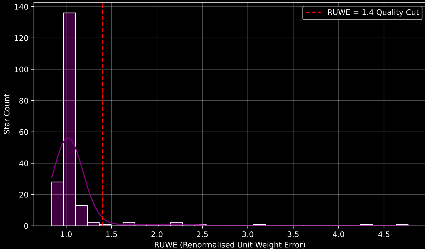
GAPOGEE DR17 Field [154+04] RUWE Distribution (n= 190)
