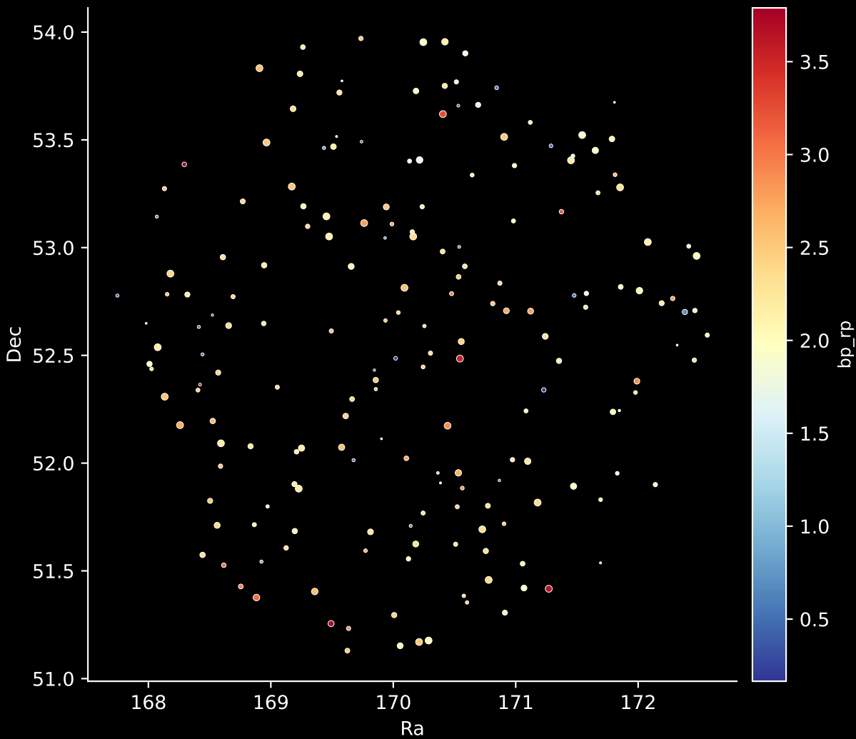
APOGEE DR17 Field: [154+04] Stars: 190
